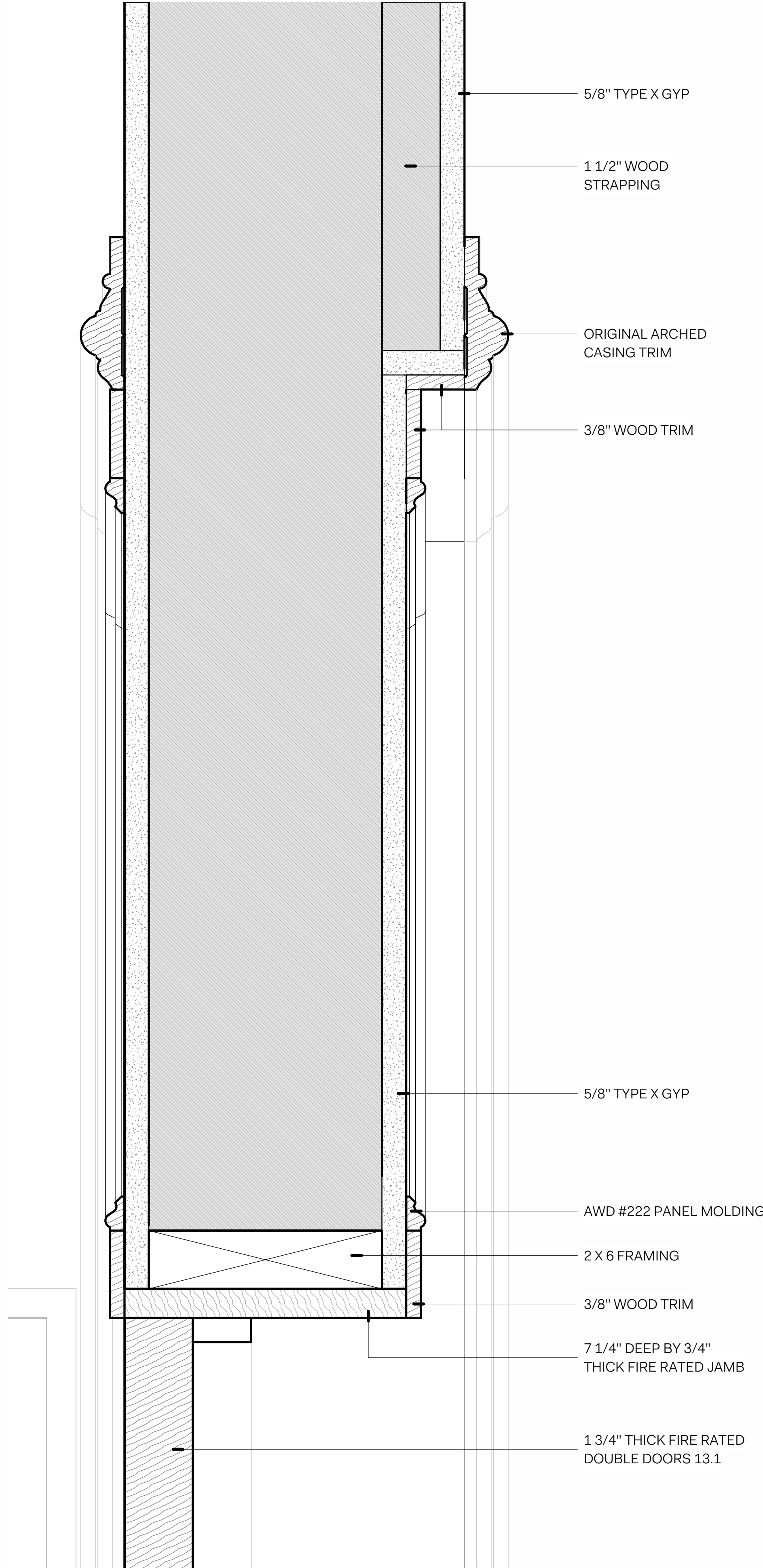
4 DOOR 13.1 TRANSOM SECTION DETAIL 6" = 1'-0"
