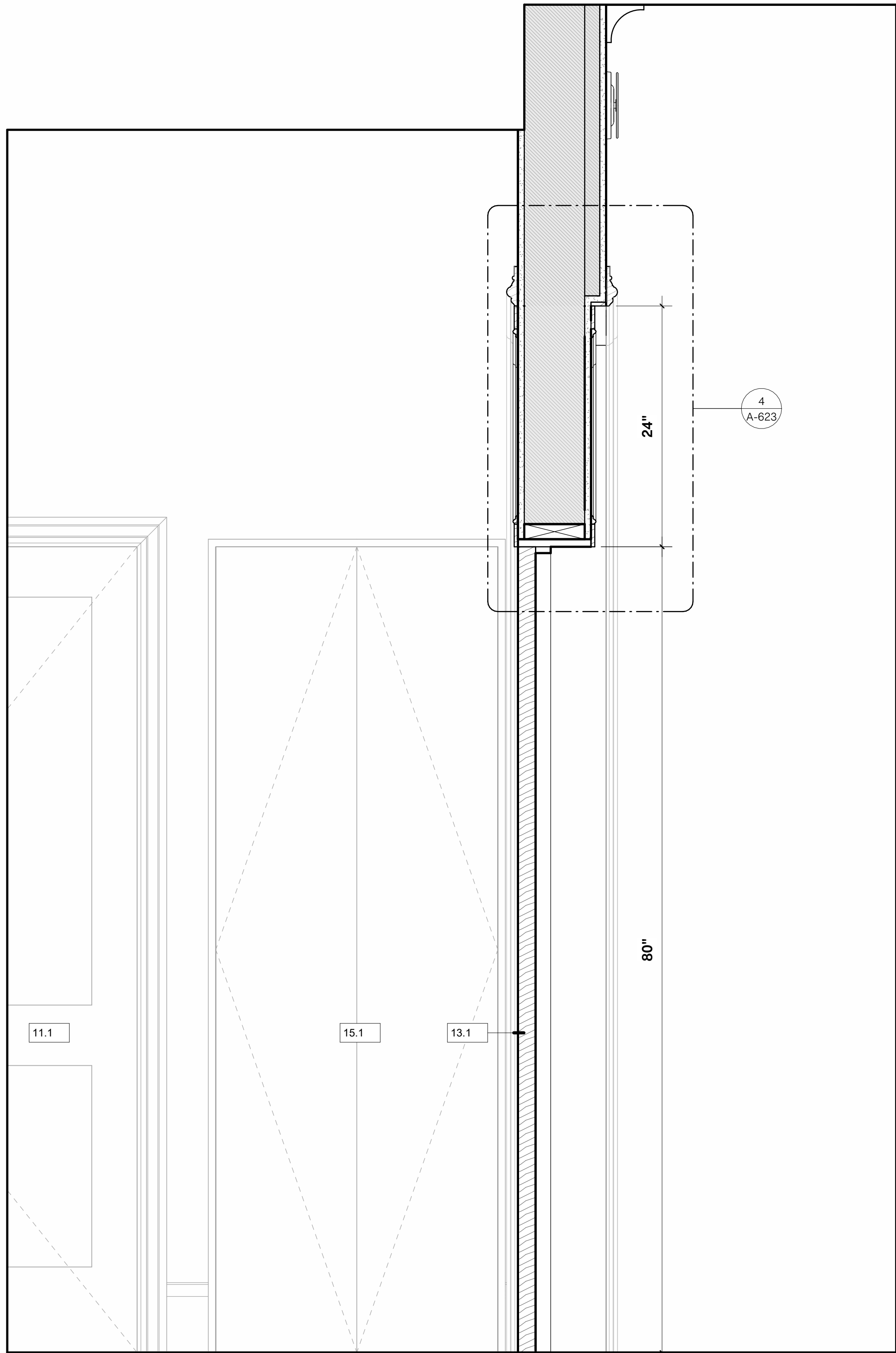
1 DOOR 13.1 SECTION DETAIL 1 1/2" = 1'-0"
