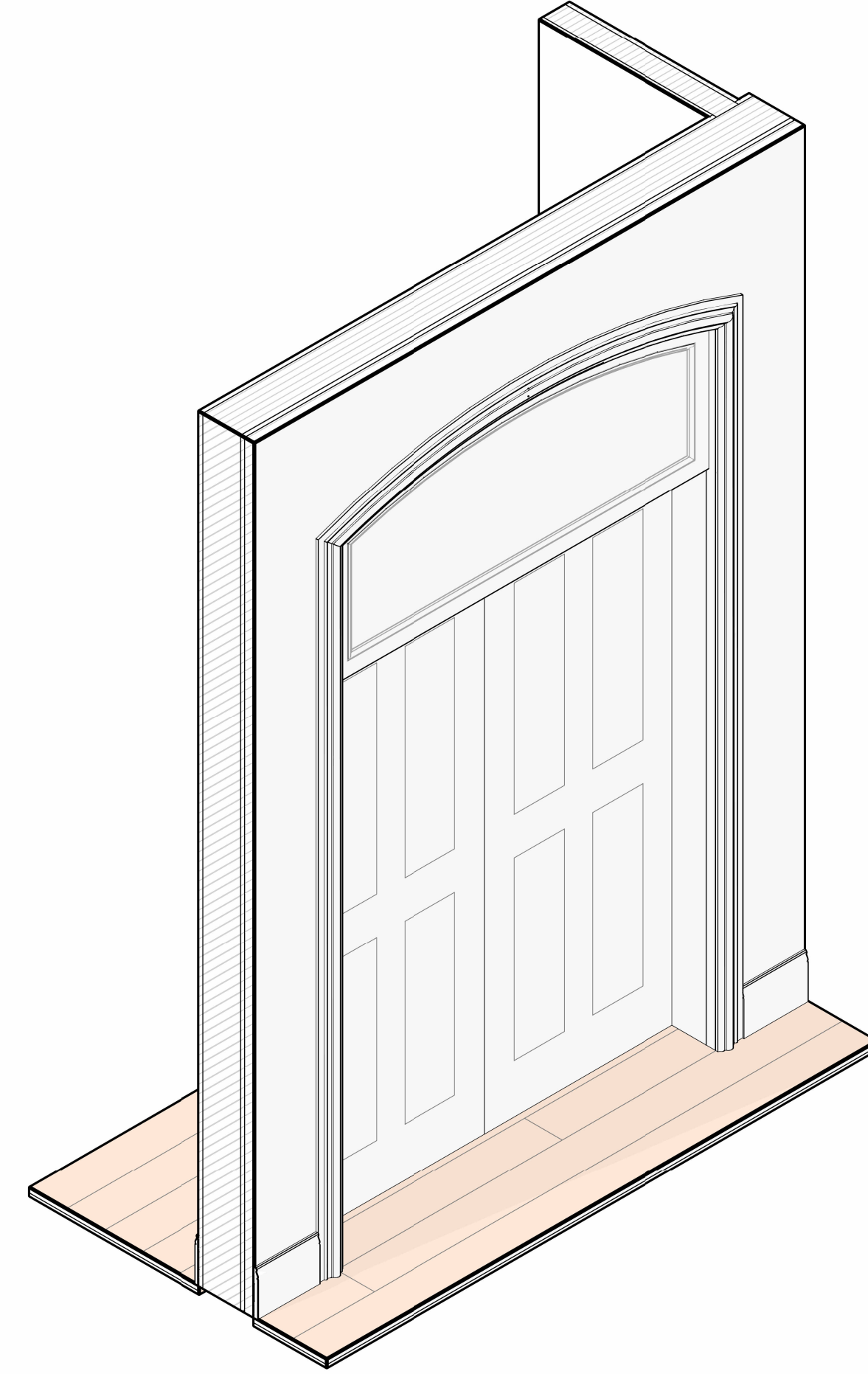
2 DOOR 13.1 - DINING ROOM SIDE AXON
